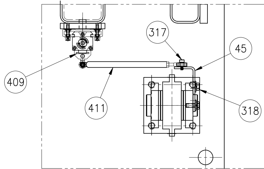
DETAIL VIEW F SCALE: 6" = 1'-0"
